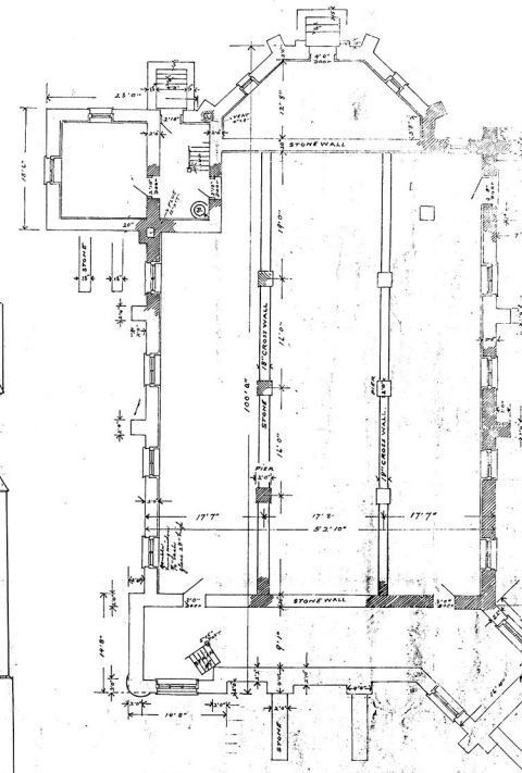
Basement and Foundation Plan 1/4" Scale
